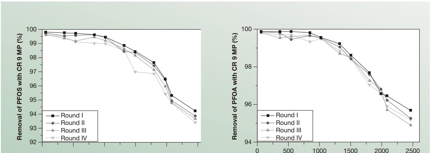
Fig. 3a and 3b Adsorption capacity after regeneration (feed concentration 50 ug/L, flow rate 20 BV/h).
