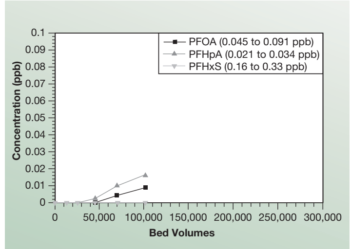
Fig. 4 Effluent readings after passing through Aldex CR 9 MP
