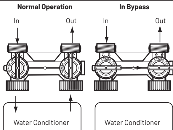
Figure 7. Model 1265 Bypass(Included)
