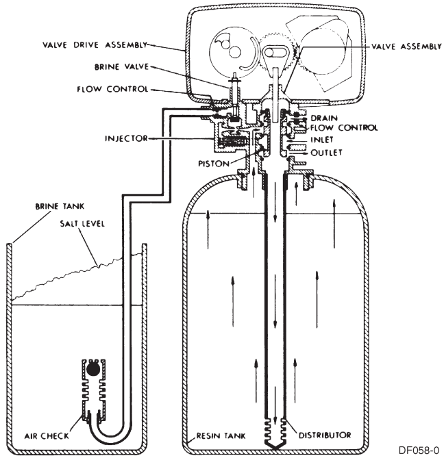
Backwash Position
