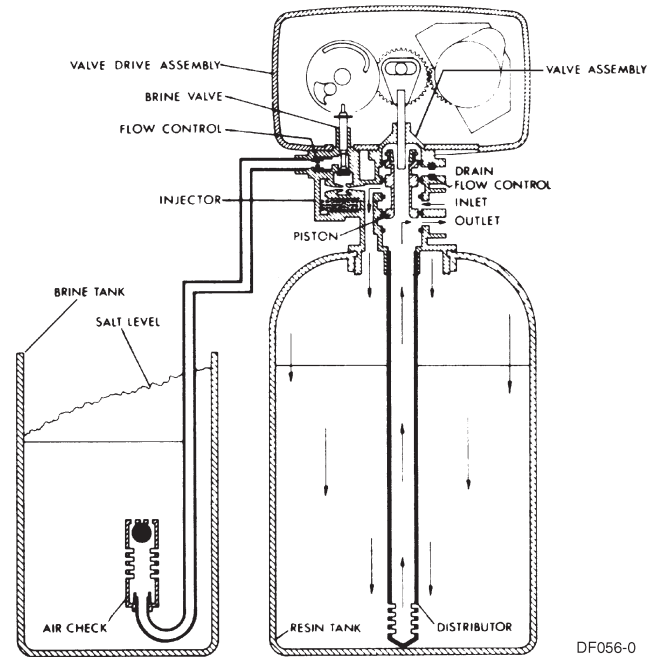
Service Position
