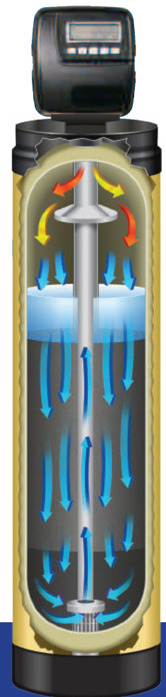
Iron Breaker III Iron & H 2 S filters
